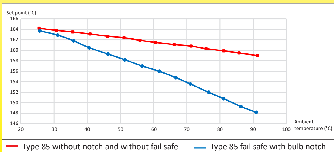
Example of a test result measuring the K/K drift for an ambient temperature variation from 25 to 90°C on a type 85 fail safe limiter calibrated at 165°C, and on the same limiter without fail safe action and without notch on the bulb
